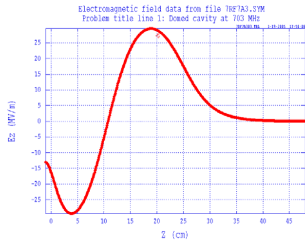
Figure 5.2 Field strength on axis of the RF gun
