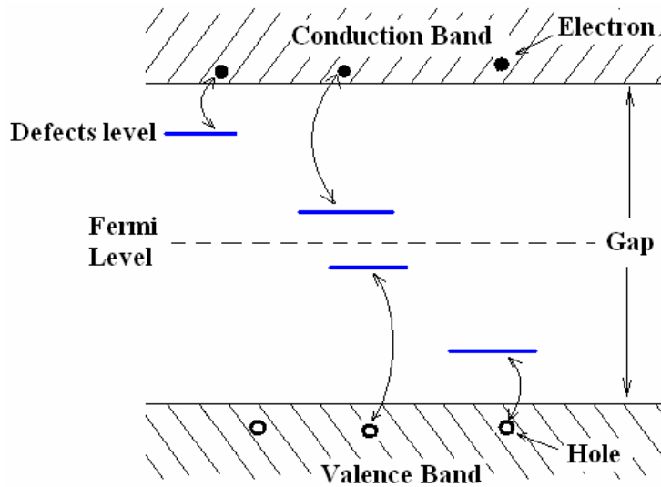
Figure 6.8 Charge carriers capture and release by excitation
