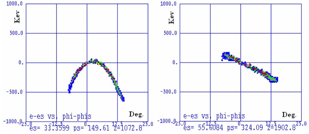
Figure 5.15 Longitudinal phase space before the 3 rd harmonic cavity and at injector exit
