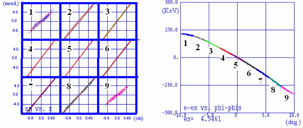
Figure 3.12 Transverse slice phase spaces (left) and longitudinal slice phase space (right) at the gun exit of the example in section 5 with \phi_0 = 60\text{deg} . Slice #1 is the front slice and slice #9 is the rear slice.
