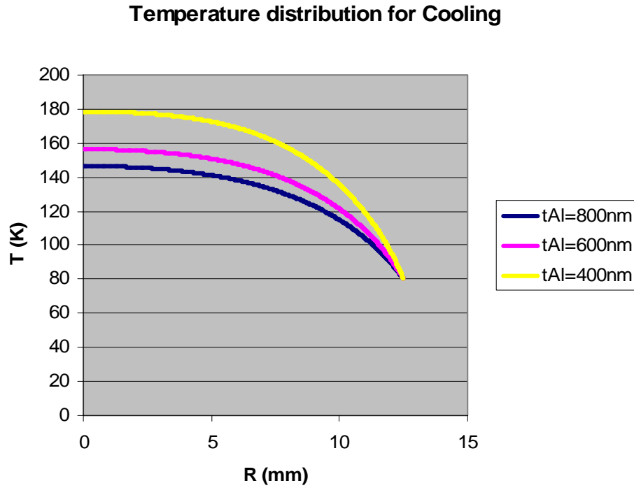
Figure 6.11 T(r) dependence on T_{Al} . The primary electron energies are adjusted according to their t_{Al} to have the same secondary electron production
