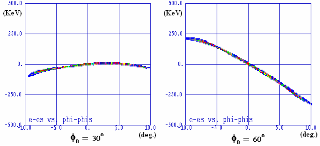
Figure 3.11 Longitudinal phase space at gun exit for \phi_0 = 30 deg. (left) and
