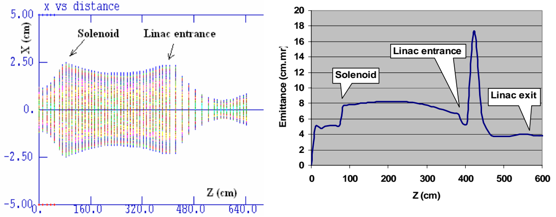
Figure 5.9 Envelope vs. z (left) & \varepsilon_M vs. z (right) of the magnetized beam
