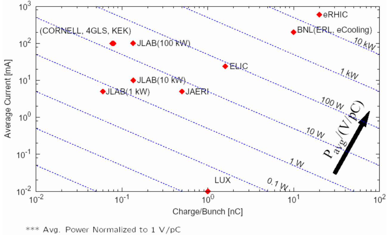
Fig. 1. HOM power as a function of bunch charge and current for a linac cavity having a loss factor of 1 V/pC.
