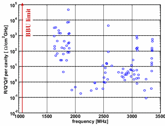
Fig.8. The dipole modes impedance multiplied by the mode frequency in GHz for the Cornell cavity.
