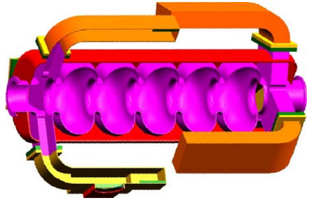
Fig. 10. The JLab ampere-class 750 MHz 5-cell cavity. Note the 3-fold symmetric layout of the 6 HOM waveguide couplers. This arrangements practically eliminates RF kicks from the couplers. The calculated monopole and dipole mode impedance of this cavity are shown in Fig. 11 and Fig. 12, respectively.
