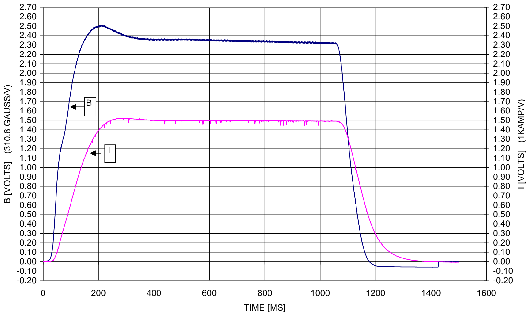
B & I VS TIME CENTER OF THIN SEPTUM MAGNET @I=1489A
