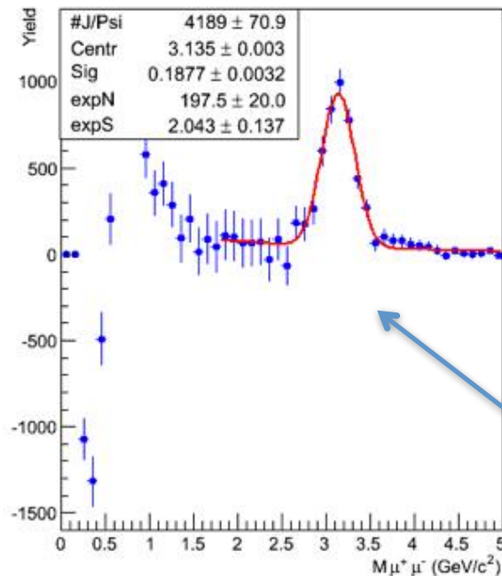
North Dimuon Mass (GeV)
