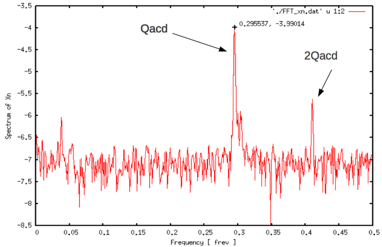
Spectrum of xn: 3Qx peak should appear at 2Qd Clearly 3Qx resonance is present in the machine.
