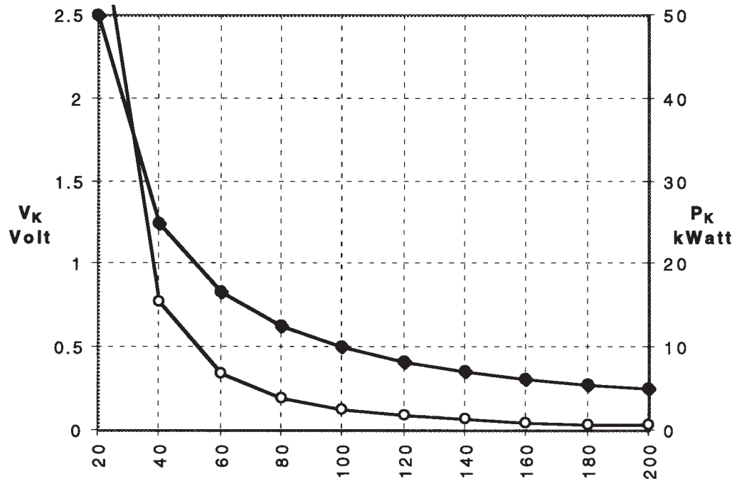
Figure 2. Kicker Voltage V_K and Power P_K vs. Damping Time \tau_D in \mu\text{s}
