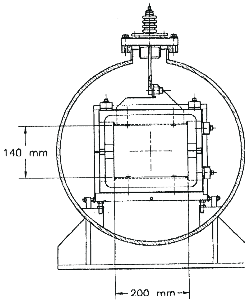
Figure 6 Lambertson & Kicker Magnet 19
