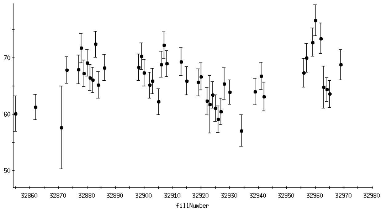
AGS Polarization by Fill
