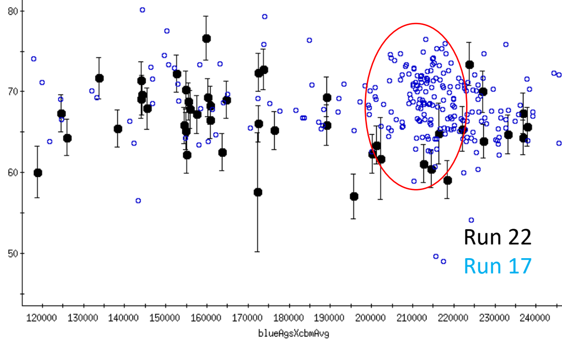
AGS Polarization by Intensity (Run 22 and Run 17)
