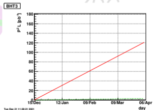
Figure: Projections for integrated luminosity
