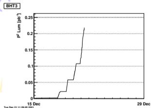
Figure: Integrated luminosity for HT3 trigger
